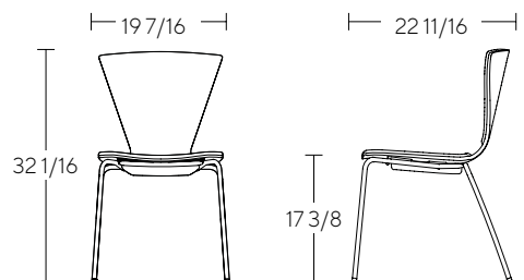
Galette Side Chair / GLS + Upholstered Seat Only / GLSU
