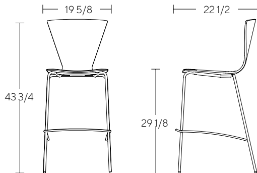
Galette Bar Chair / GLB + Upholstered Seat Only / GLBU
